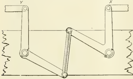
A SIGNAL PIPE-LINE COMPENSATOR.
